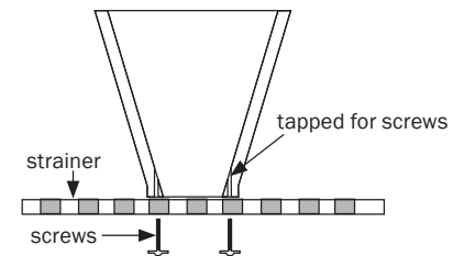
863-FN installation
